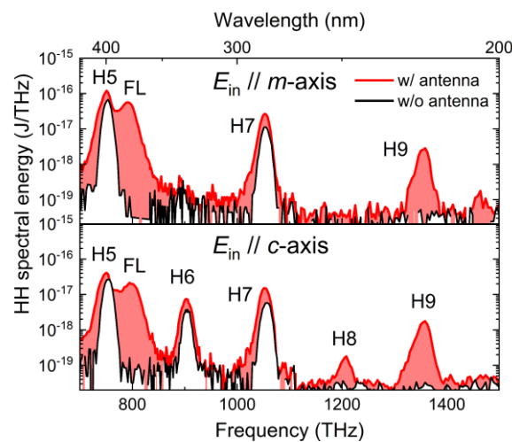
Fig. 2. (a, b) HH spectra measured at input intensity of 0.10 TW/cm 2 for (a) the sample I ( E_{in} // m -axis) and (b) the sample II ( E_{in} // c -axis). The red (black) lines indicate the HH spectra generated from ZnO with (without) antennas.
