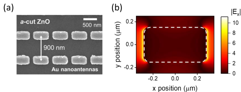
Fig. 1. (a) A SEM image of an antenna array fabricated on ZnO. (b) A simulated near-field distribution of |E_x| inside the ZnO substrate (2-nm beneath the air-ZnO interface). The dashed line shows the antenna area.
